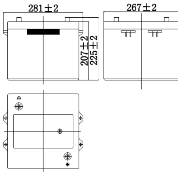
Dimensions for casing
